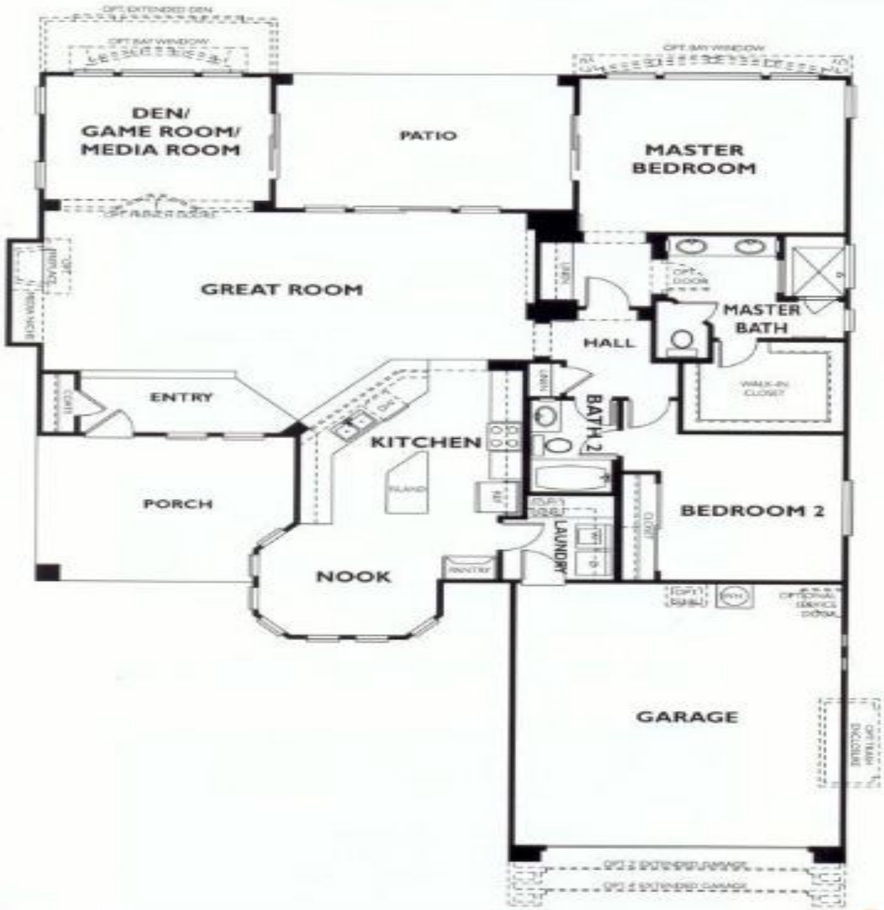
Trilogy Novus Floorplan - no Casita
